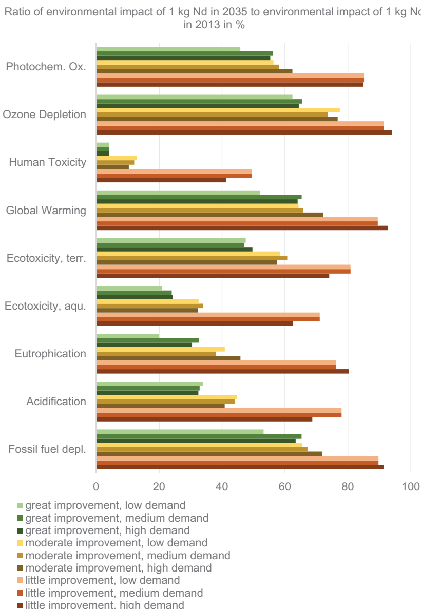
FIGURE 3 Ratio of environmental impacts of 1 kg Nd in 2035 to environmental impacts of 1 kg Nd in 2013. Values for 2035 are taken from nine future scenarios resulting from a combination of sub-scenarios. “Improvement” summarizes assumptions on the future success of the Chinese consolidation strategy as well as environmental improvement of background processes. Demand relates to the future global demand for these metals, which affects the environmental impact of 1 kg of metal by influencing the contribution from different mining sites. Underlying data used to create this figure can be found in Supporting Information S3a
