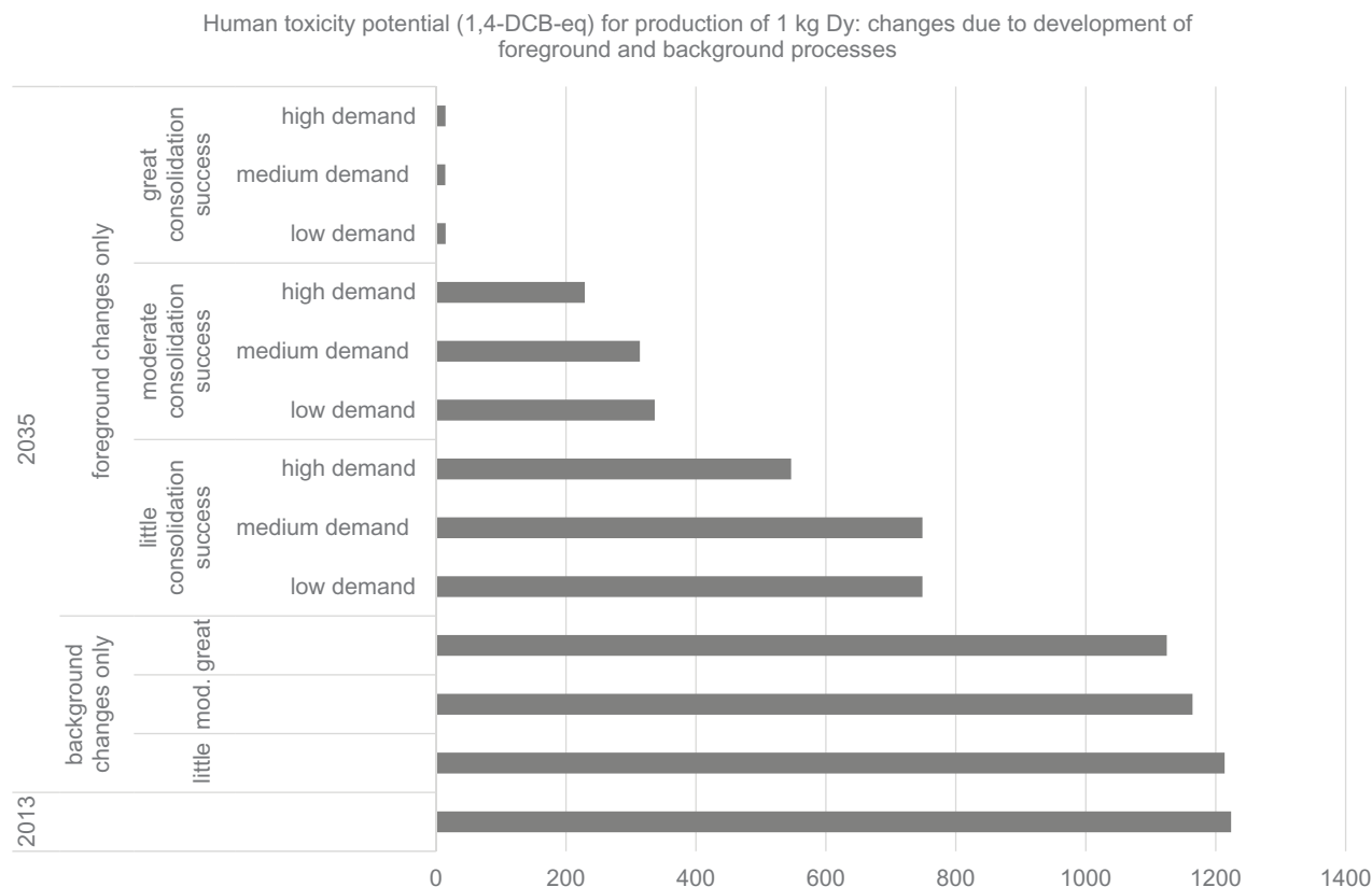
FIGURE 5 Comparison of changes in the human toxicity potential of producing 1 kg Dy due to changes in the background system versus changes in the foreground system. Underlying data used to create this figure can be found in Supporting Information S3b
