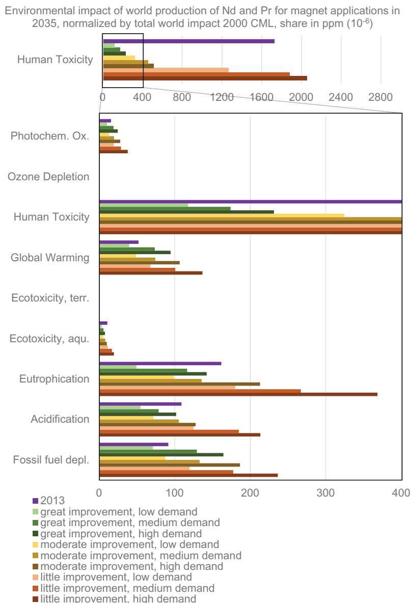
FIGURE 6 Environmental impact of world production of Nd and Pr for magnet applications in 2013 and in 2035. All values are normalized using CML data sets for the overall global impacts in the considered impact categories in 2000 (van Oers, 2015), shares are given in parts per million (ppm). Values for 2035 are taken from nine future scenarios resulting from a combination of sub-scenarios. "Improvement" summarizes assumptions on the future success of the Chinese consolidation strategy as well as environmental improvement of background processes. Demand describes the future global demand for these metals. Underlying data used to create this figure can be found in Supporting Information S3a and S3c
