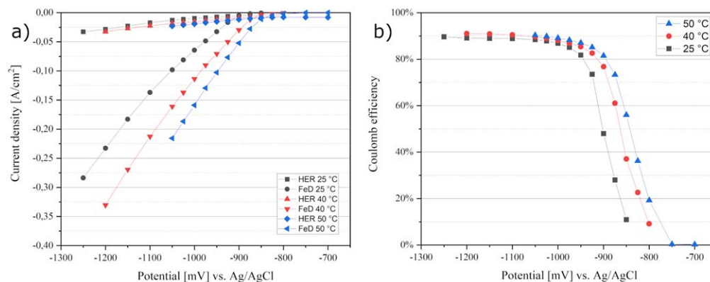
Figure 4. Quantitative anodic stripping voltammetry recorded on poly-Au RDE rotating at 2000 rpm in electrolyte with composition 2.0 M NH 4 Cl, 1.5 M FeCl 2 , pH = 2.0. (a) Partial current density vs applied potential at different temperatures for HER and Fe deposition; (b) Coulombic efficiency vs potential. Each data point is the average of four measurements.
