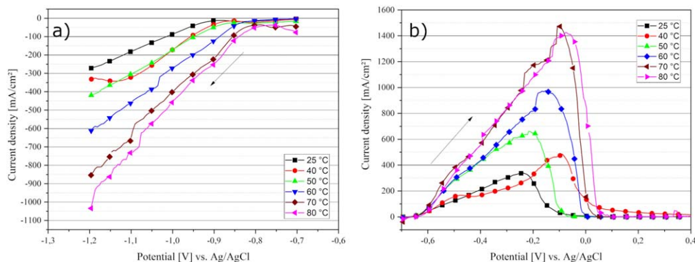
Figure 3. Linear sweep voltammograms on poly-Au WE pre-plated with Fe from pH = 2.4 solution of 1.5 M FeCl 2 and 2.0 M NH 4 Cl. After plating for 30 s at −1.2 V, the potential was swept from −0.7 V in the cathodic (a) or anodic (b) direction at a sweep rate of 20 mV s −1 .
