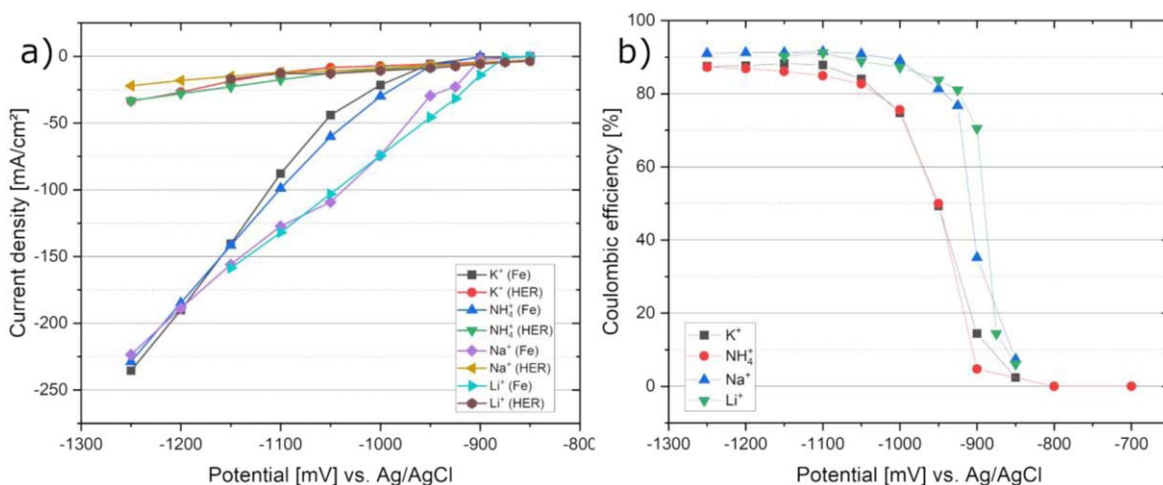
Figure 11. Partial current density of HER and Fe deposition (a), and the corresponding coulombic efficiency (b). Data obtained by quantitative anodic stripping voltammetry method on a Au RDE rotating at 2000 rpm, with plating time of 30 s, in electrolyte of 2.0 M XCl, 1.5 M \text{FeCl}_2 , pH = 2.0. Each data point is the average of four scans.
