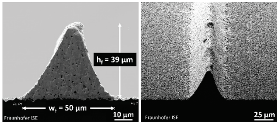
Figure 5: SEM images of contacts with triangular shape printed with LIDE-structured glass foil stencils.
