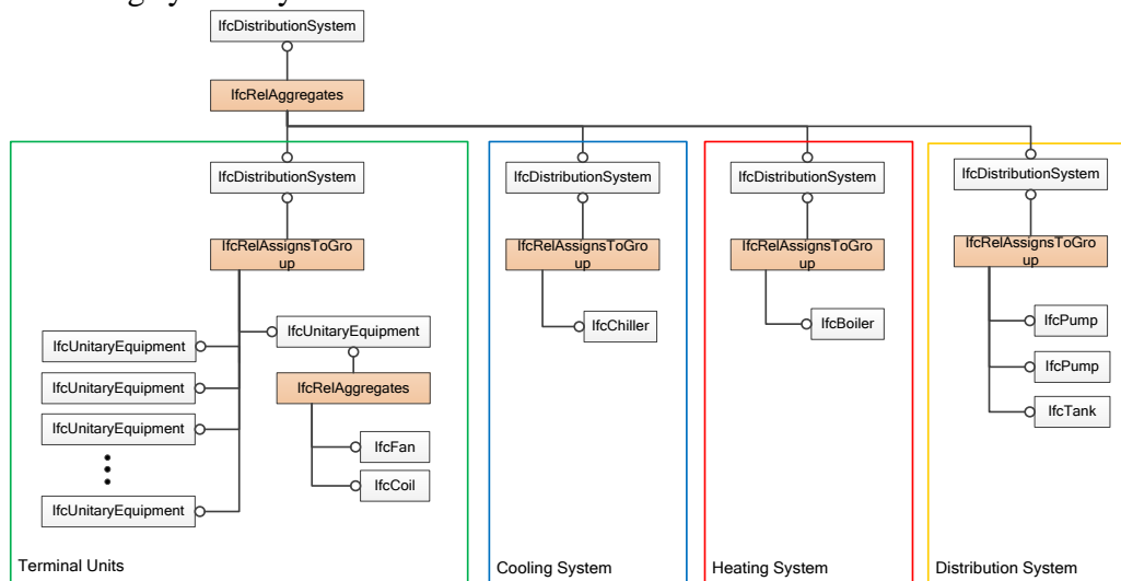
Figure 5.8: EXPRESS-G - System aggregation
