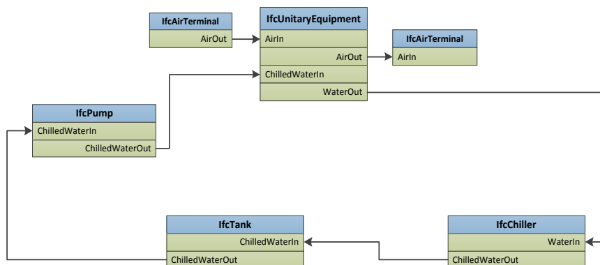
Figure 5.7: Illustration of the port connection
