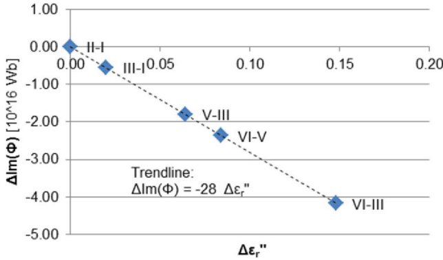
Fig. 5. Change of imaginary part of the magnetic flux passing through the coil showing a negative linear dependence on the change of the imaginary part of permittivity for nonconductive samples.
