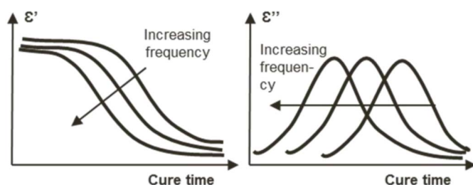
Fig. 6. Progress of complex permittivity during cure [38], [39].
