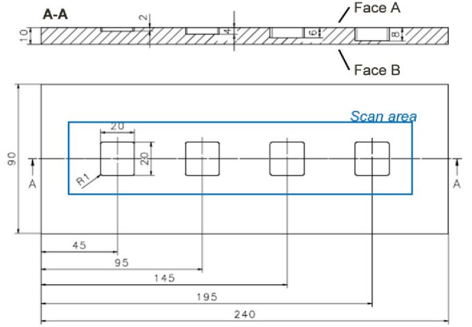
Fig. 13. Specification of sample 2, measures in millimeter.
