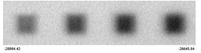
Fig. 14. HFEC image of sample 2, face A. Measurement values in digits.
