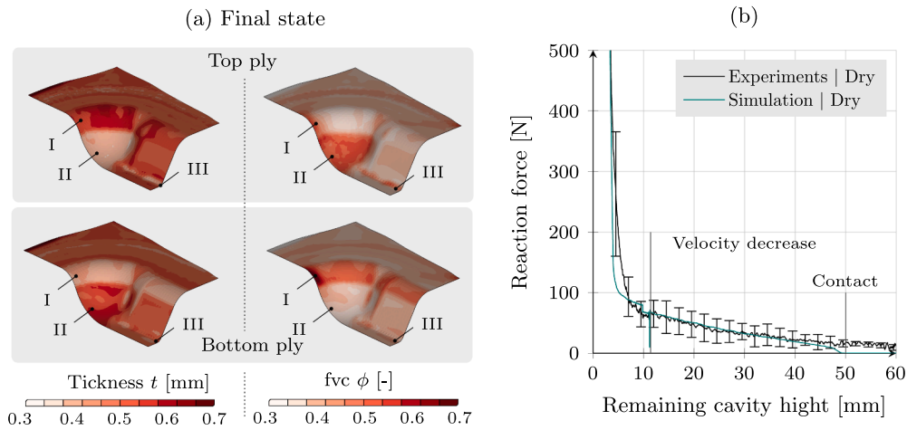
Fig. 17. Forming submodel | (a) Thickness t and \text{fvc } \phi for closed mould; (b) Reaction forces.
