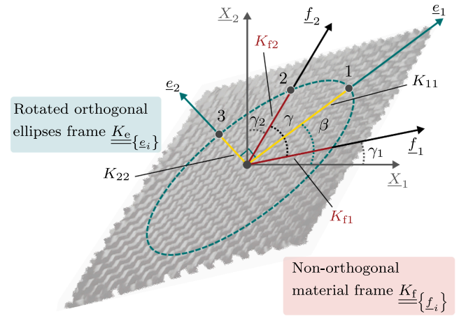
Fig. 3. Permeability modelling | Illustrational orthogonal and non-orthogonal frames during "pure shear" deformation. Three points are needed to for a unique reconstruction of the ellipse.
