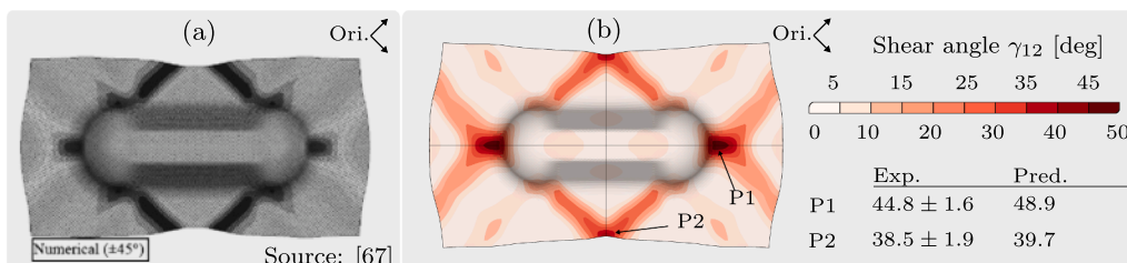
Fig. 16. Forming submodel | (a) Shear angle distribution provided by Boisse et al. [67]; (b) Shear angle distribution in the present work and direct comparison with own experiments at two critical points (P1,P2).
