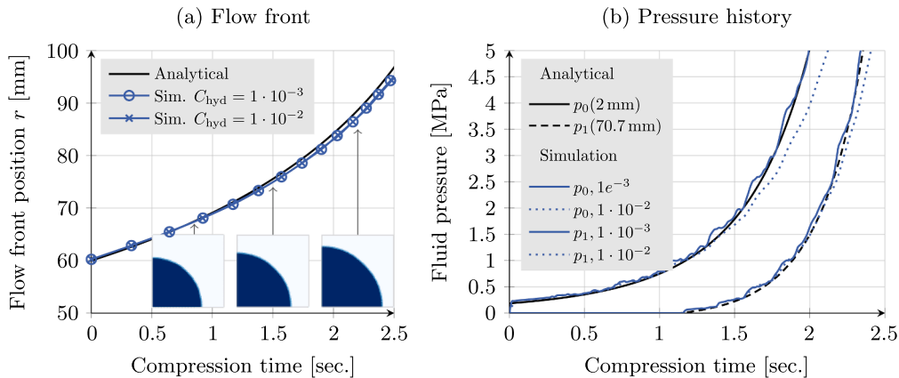
Fig. 12. Compaction test case | Comparison with analytical solution: (a) Flow front progression; (b) Discrete pressure history at p_0(2 \text{ mm}) and p_1(70.7 \text{ mm}) for two hydraulic capacities.
