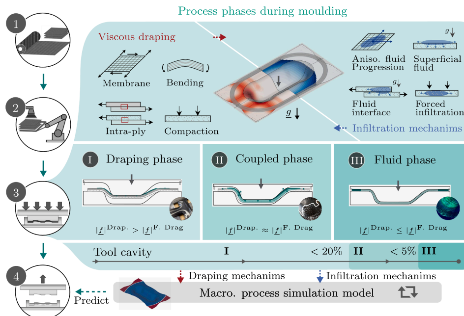
Fig. 1. Graphical abstract | WCM process steps, crucial mechanisms and aim of this study.
